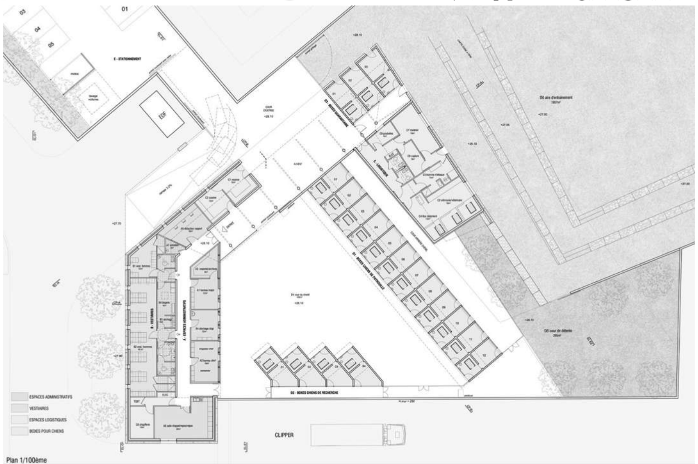
Imagen 27. Planta arquitectónica Canine Brigade. Fuente: http://www.archdaily.com/195081/canine-brigade-transform-ds-architecture/5004cad128ba0d4e8d00026e-canine-brigade-transform-ds-architecture-plan-01
