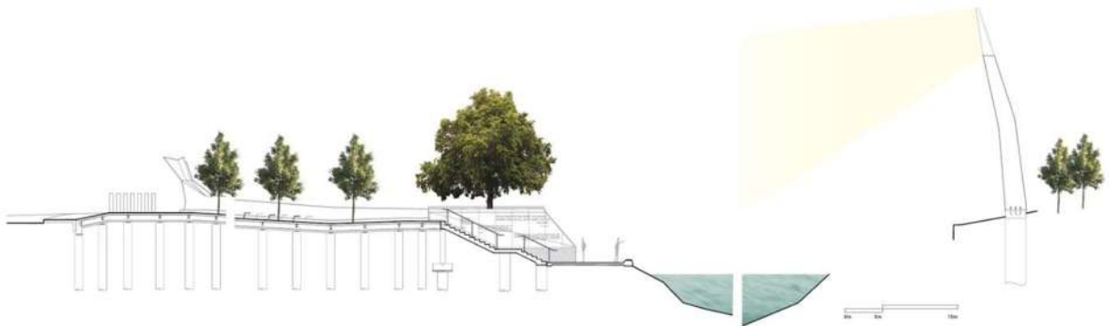
Ilustración 31. Plaza Poppy/ The Marc Boutin Architectura, corte, recuperado de https://www.archdaily.mx/mx/785658/plaza-poppy-the-marc-boutin-architectural-collaborative/56fb3cb0e58ecebba500004c-poppy-plaza-the-marc-boutin-architectural-collaborative-section?next_pro
