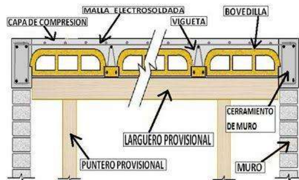
Fig. 32. Proceso constructivo de losa de vigueta y bovedilla, https://www.google.com/url?sa=i&url=https%3A%2F%2Fwww.arqhys.com%2Fcasas%2Fmuro-tabique.html&psig=AOvVaw3awmoF2BQnbmtYCTTp9A16&ust=1592623485758000&source=images&cd=vfe&ved=0CA0QjhxFwoTCNC_nfz2jOoCFQAAAAAdAAAAABAD , F de Rec 11/19.
