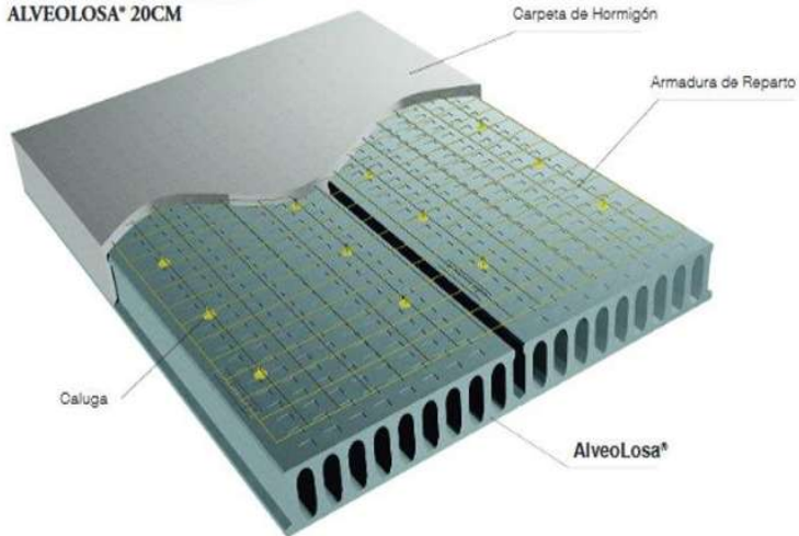
Fig.33. tipos de losa para techos, https://www.google.com/url?sa=i&url=https%3A%2F%2Fingenieria.yogameok.com%2Flos-5-tipos-de-losas-techos%2F&psig=AOvVaw0s4yESKLifcRziulxgcqKI&ust=1592621389341000&source=images&cd=vfe&ved=0CA0QjhxFwoTCKjAkZ7vjOoCFQAAAAAdAAAAABAt . F de Rec 11/19.
