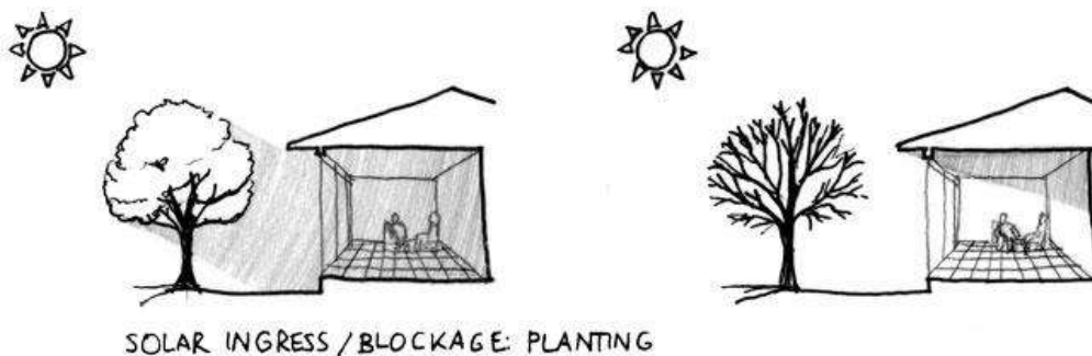
Fig. 6. Enfriamiento y calentamiento. https://images-blogger-opensocial.googleusercontent.com/gadgets/proxy?url=http%3A%2F%2Fwww.botanicaatlanta.com%2Fsummer-winter-solar-ingress-planting.jpg&container=blogger&gadget=a&rewriteMime=image%2F F. de Rec. 11/19
