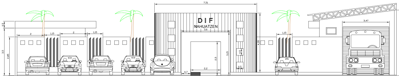
FACHADA PRINCIPAL
